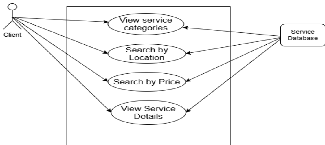
Figure 3: Level 2.2 for Local Service management system
