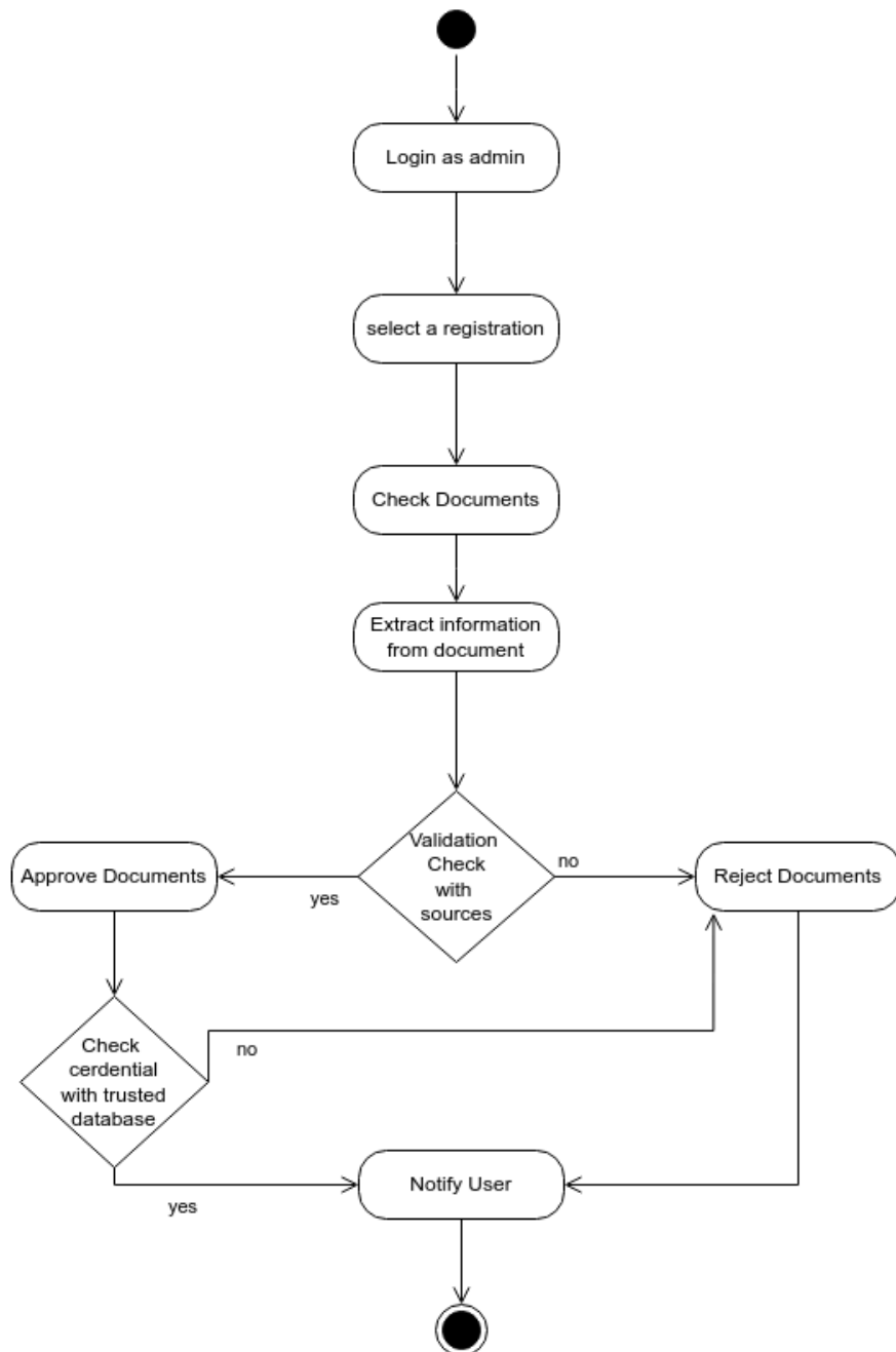
Figure 30: Activity Diagram for Verify documents credentials
