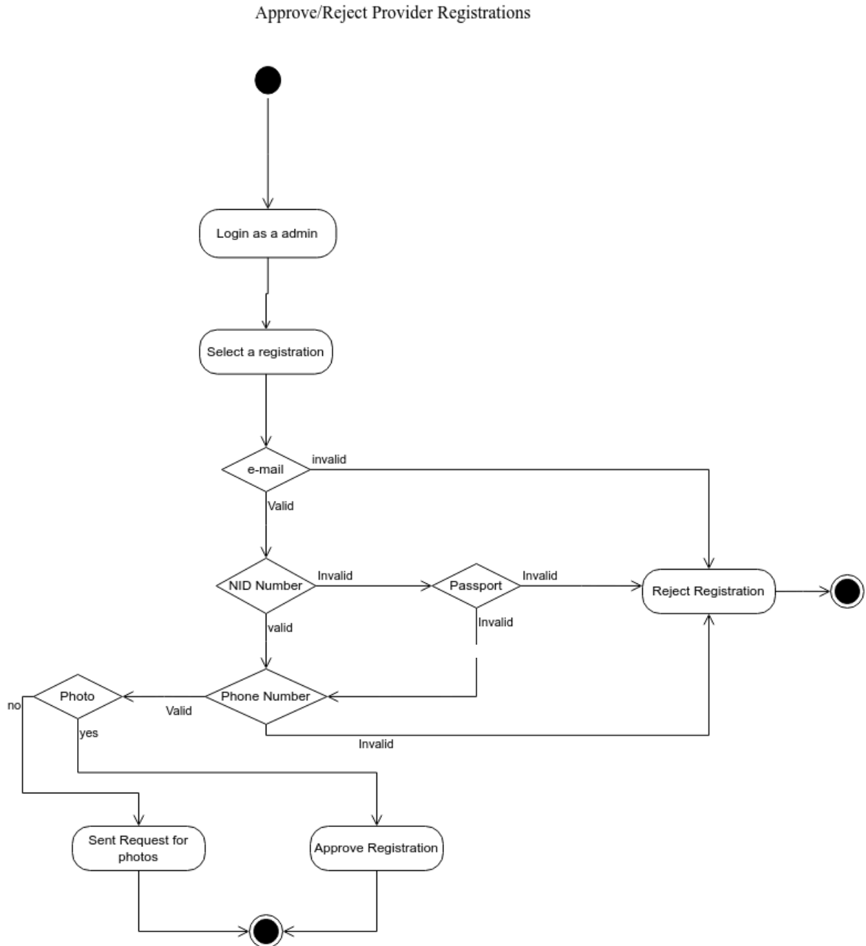
Figure 26: Activity Diagram for Approve/Reject Provider Registrations
