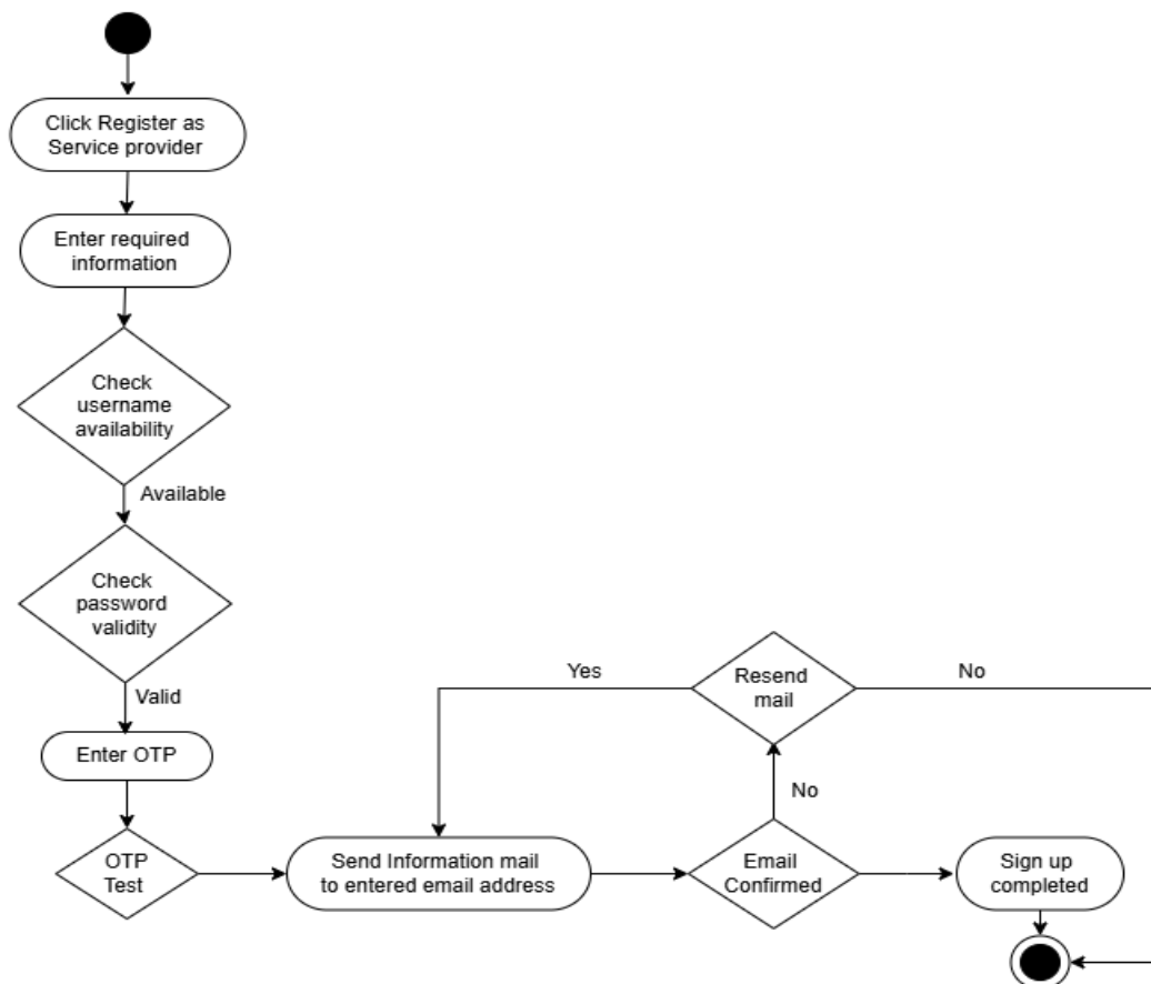
Figure 10: Activity Diagram for Register as service provider
