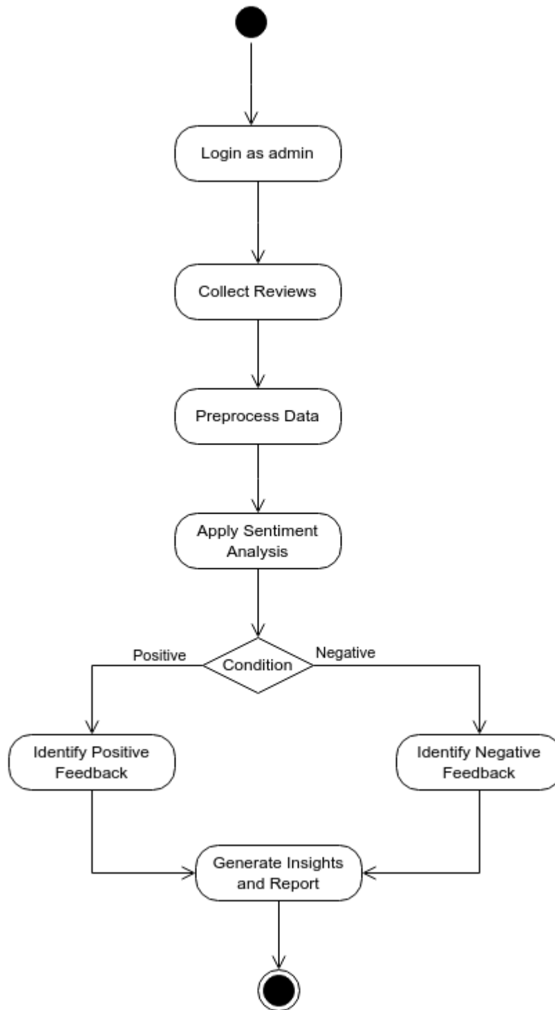
Figure 33: Activity Diagram for Analyse Reviews
