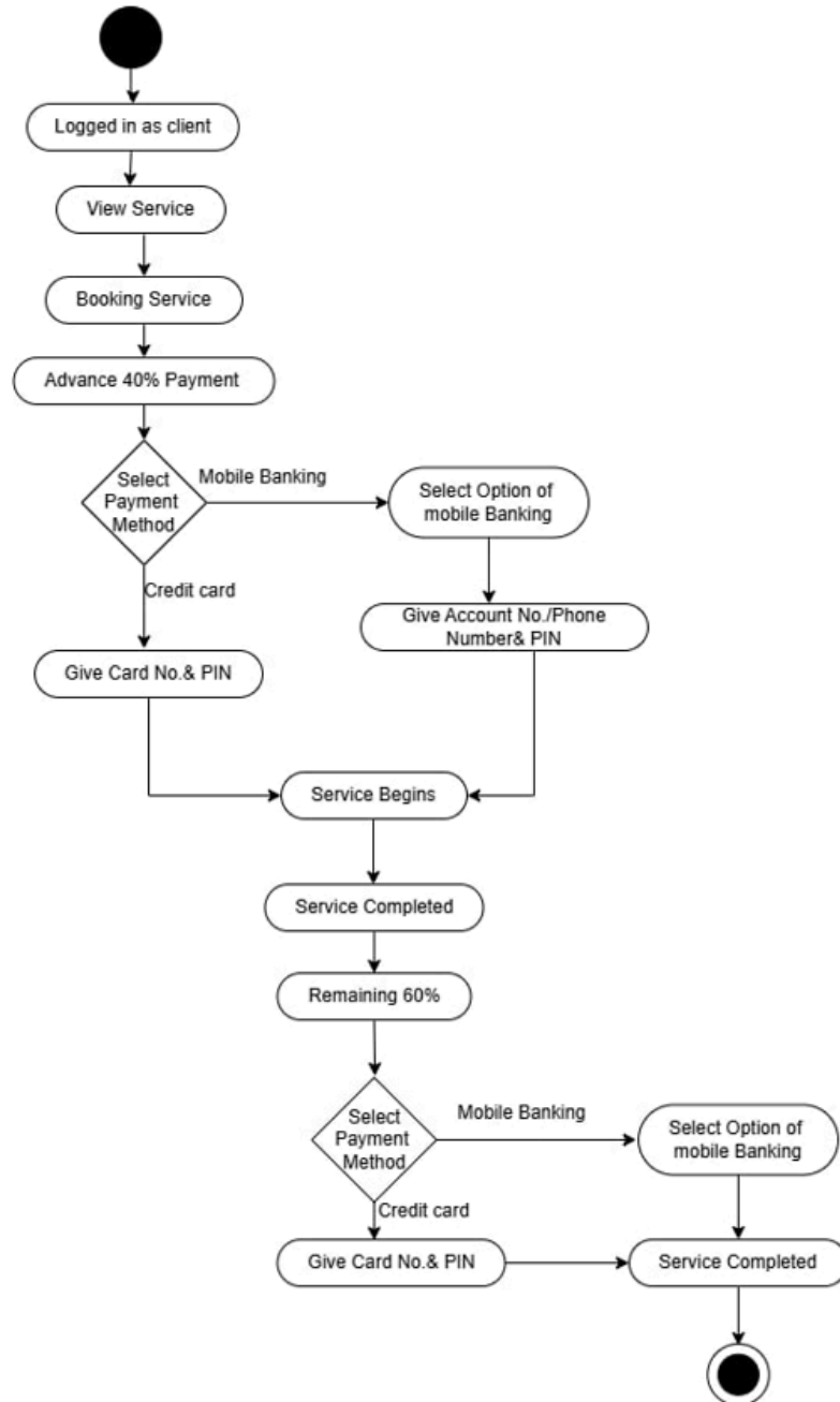
Figure 22: Activity Diagram for Select Payment Method
