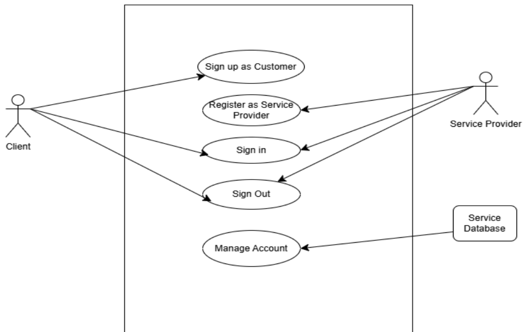
Figure 2: Level 2.1 for Local Service management system
