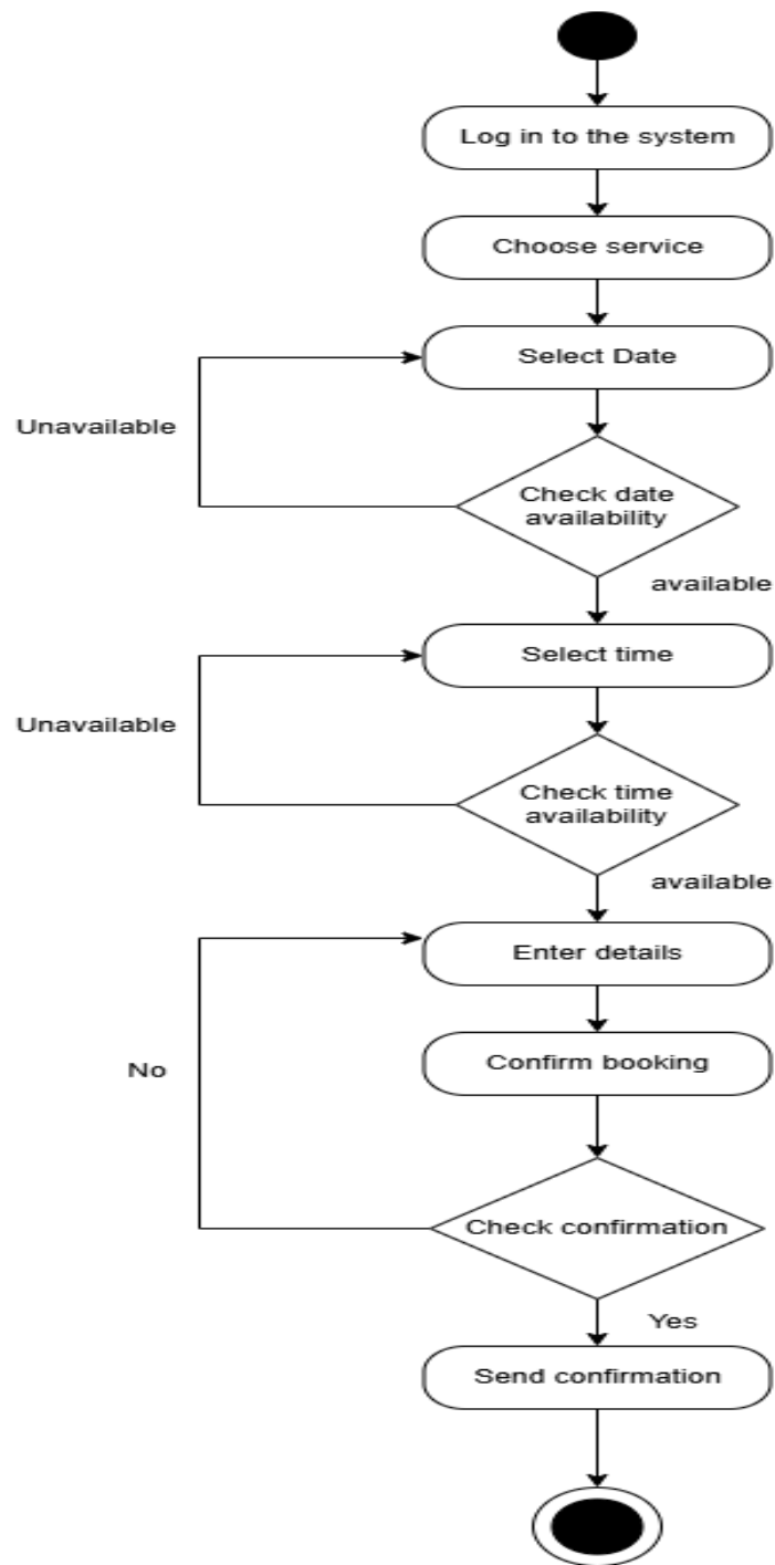
Figure 20: Activity Diagram for Confirm Booking
