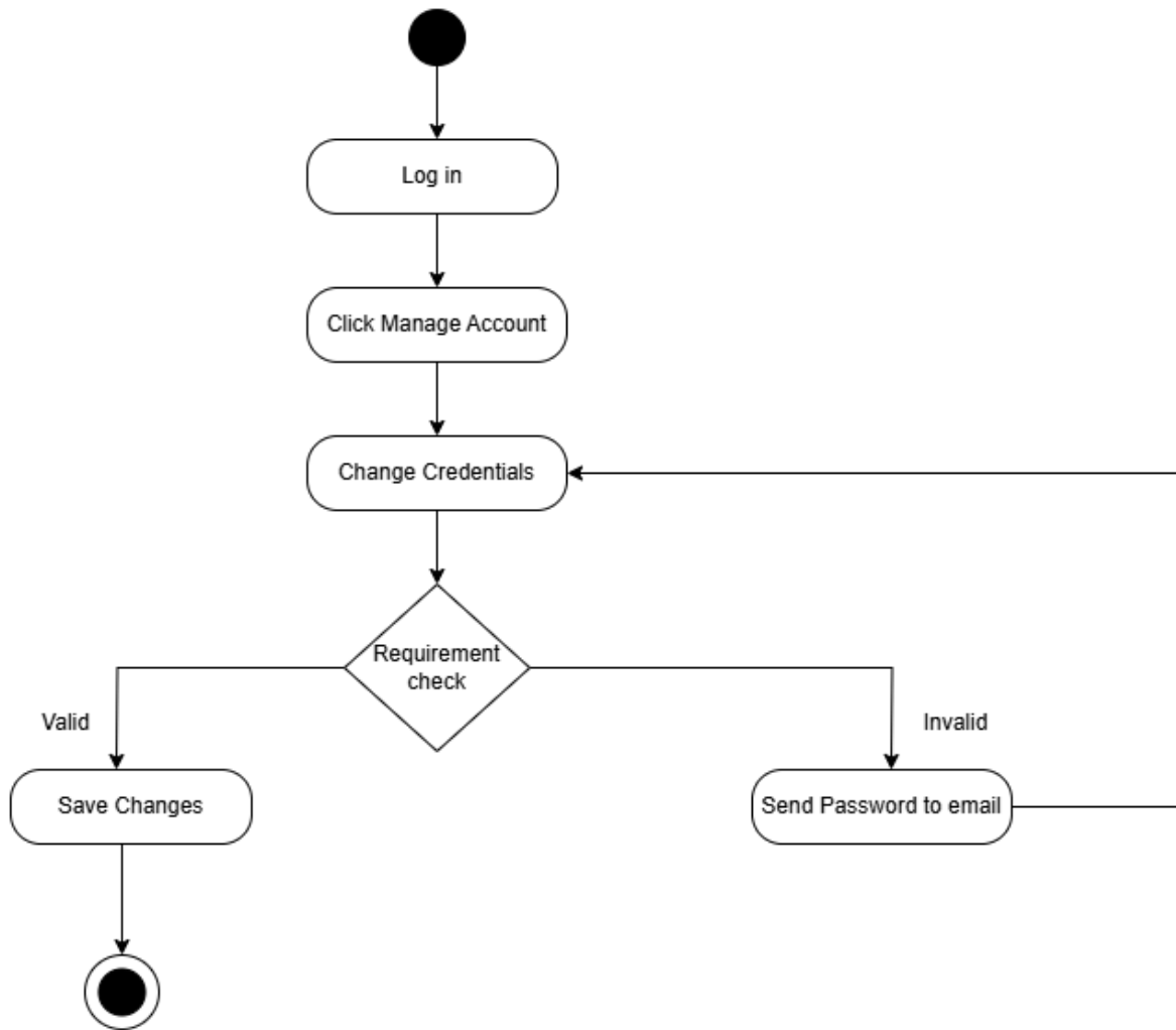
Figure 14: Activity Diagram for Manage Account
